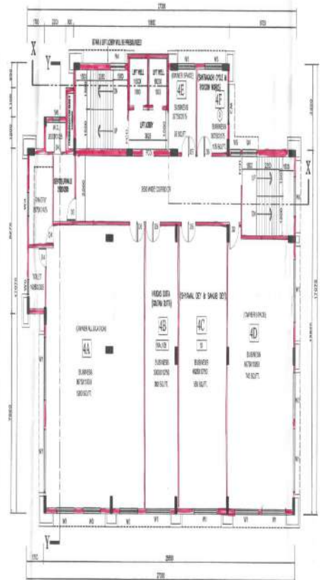
PROPOSED FOURTH FLOOR PLAN SCALE: 1/8" = 1'-0" (OWNER & TENANT REHABILITATION)
