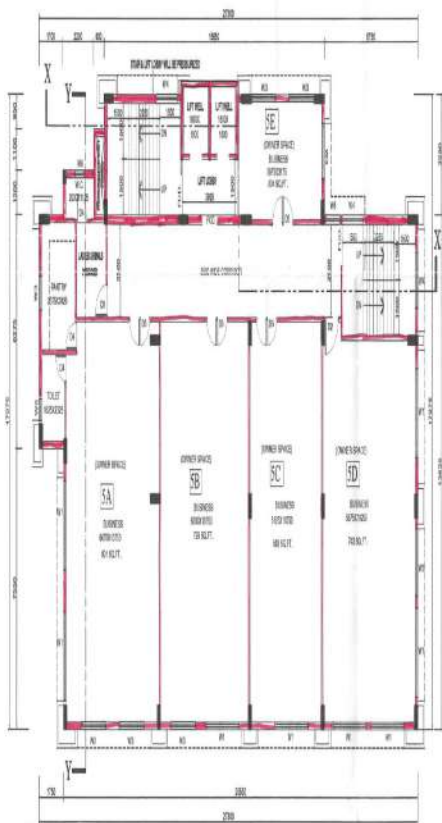
PROPOSED FIFTH FLOOR PLAN SCALE: 1/8" = 1'-0" (OWNER REHABILITATION)
